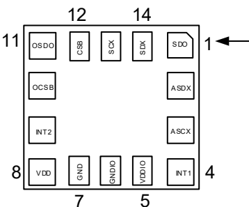
LGA14-2.5x3x1.00mm 3 (仰视图)
