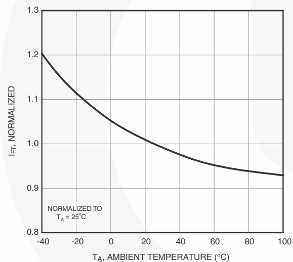
Figure 5. Trigger Current vs. Temperature
