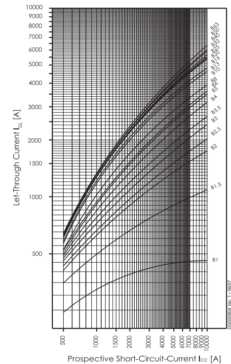
Type B (IEC/EN60898)
