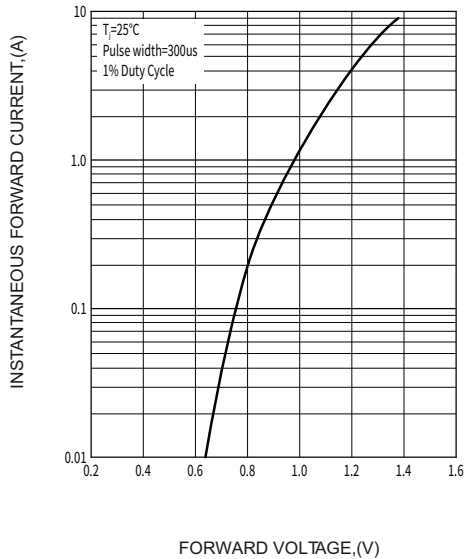
FIG.1-TYPICAL FORWARD CHARACTERISTICS
