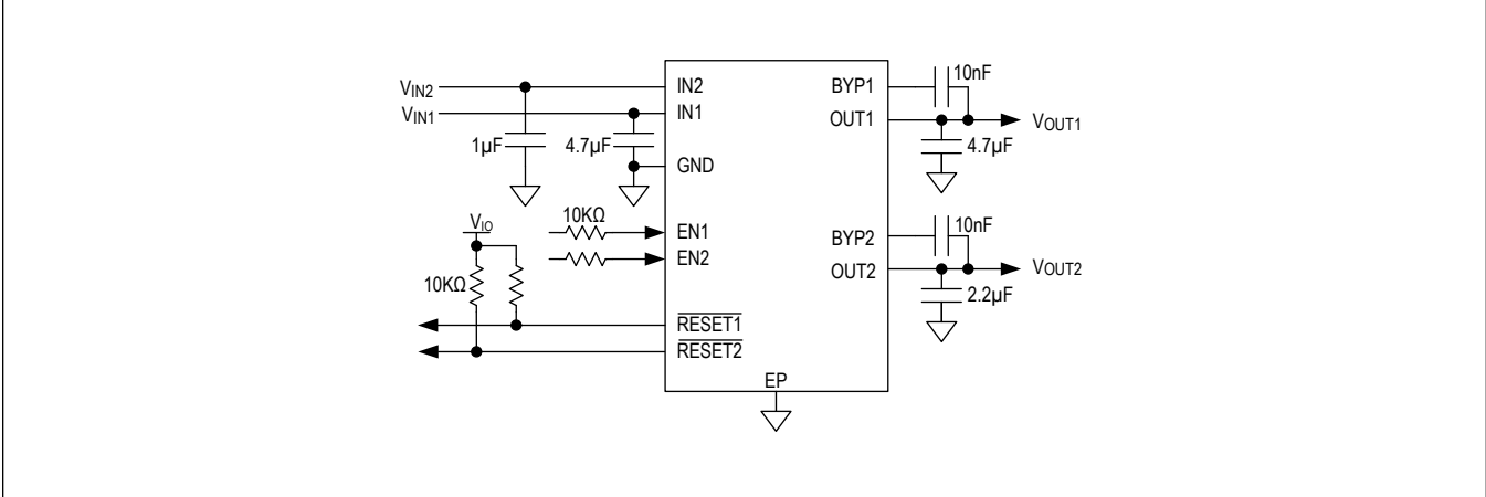
Circuit 2 (MAX25307)
