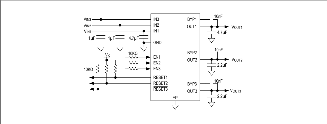
Circuit 2 (MAX25307)
