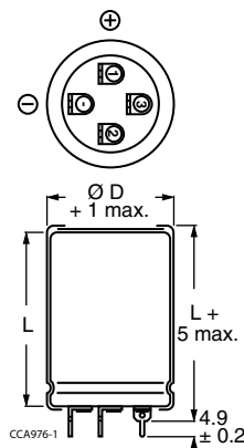
Fig. 2 - Printed wiring pin version (Case \varnothing D = 35 mm)
