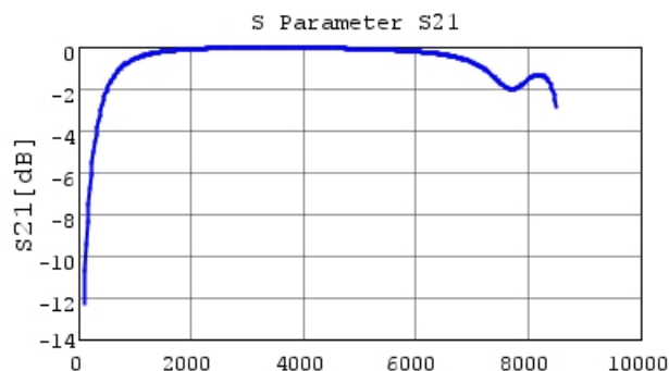
GRM1885C2A4R0CA01 S21 DCOV, 25degC
