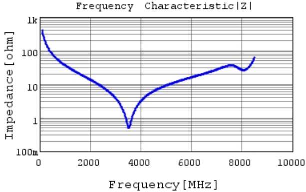
GRM1885C2A4R0CA01 |Z| DCOV, 25degC
