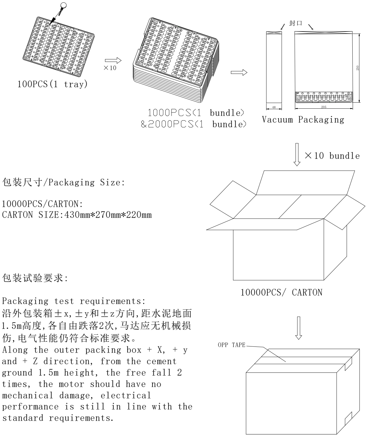
Pack drawing of Vibrator Motor
