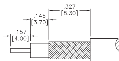
RECOMMENDED STRIPPING DIMENSIONS
