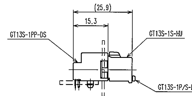
MATED CONNECTOR
