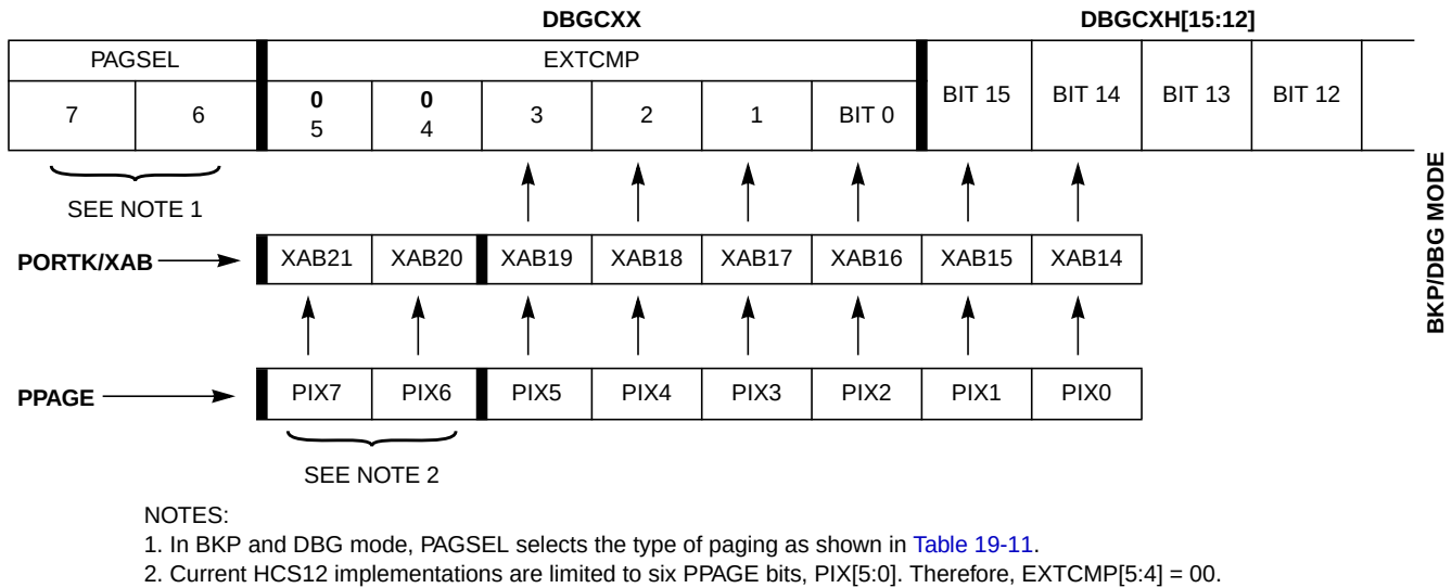
Figure 19-10. Comparator C Extended Comparison in BKP/DBG Mode
