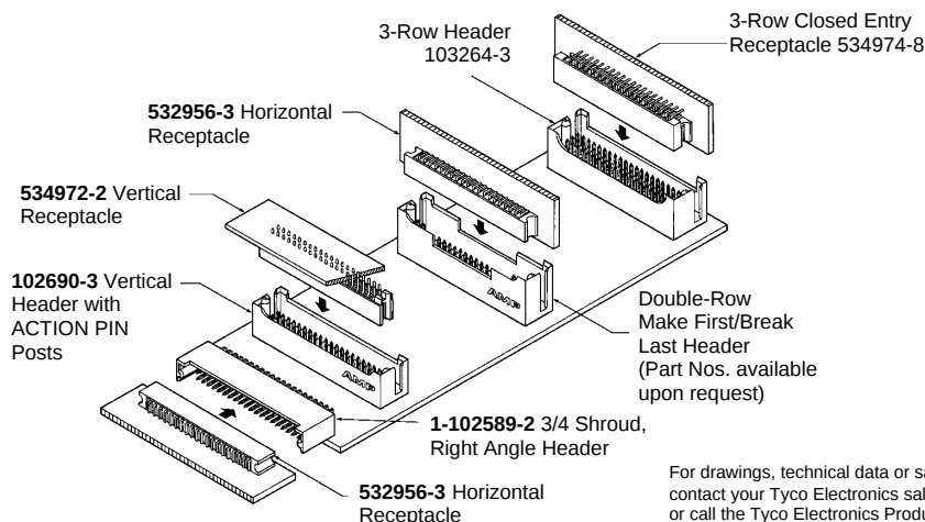
Receptacle Contact (Double Beam with Anti-Overstress) Board Retention Feature Available
