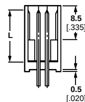
Section X-X
