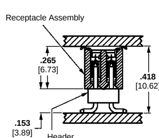
Figure 3 Double-Row, Mod IV, Surface-Mount, Top Entry, Receptacle and Surface-Mount Breakaway Header
