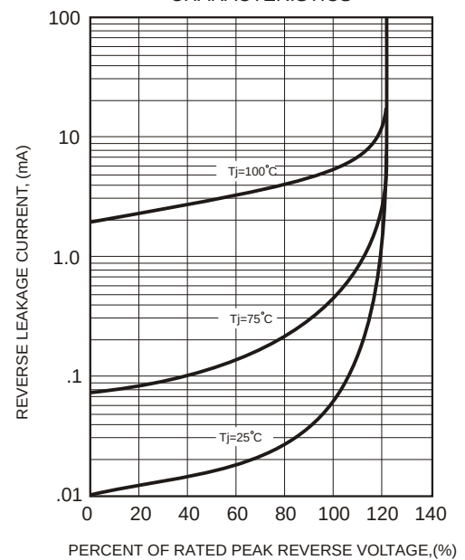
FIG.5 - TYPICAL REVERSE
