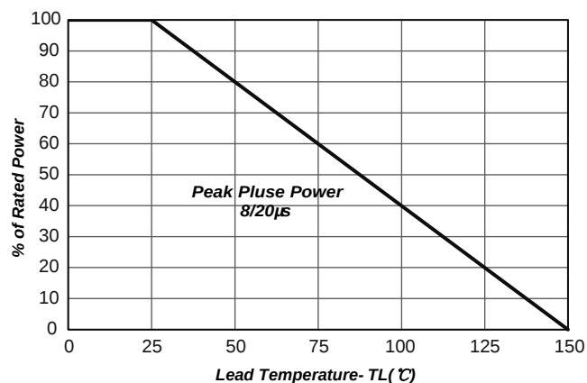
Fig2. Power Derating
