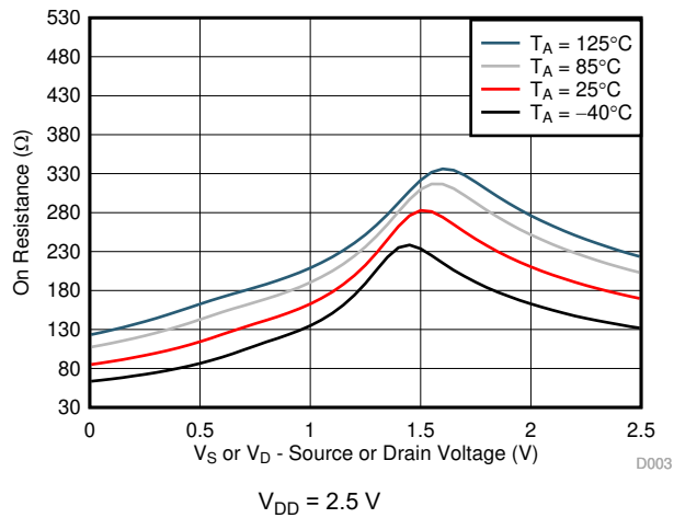
Figure 7-3. On-Resistance vs Temperature
