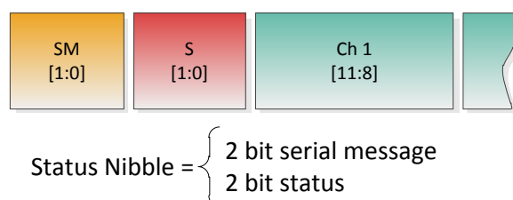
fig. 17 - SENT Status Nibble and Serial Message
