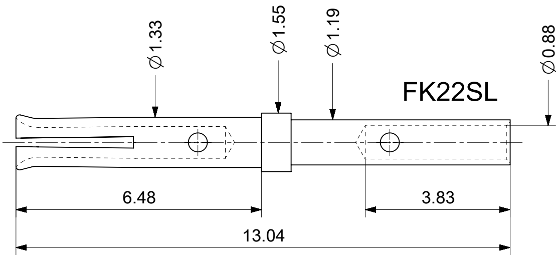
SOCKET Material: Copper alloy
