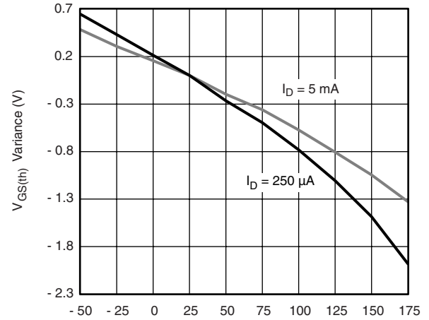
Threshold Voltage
