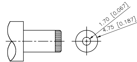
MATING PLUG Jack Insertion Depth: 8.5 mm
