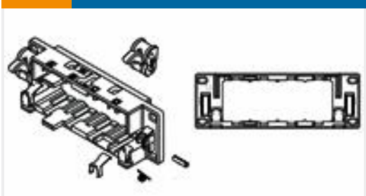
TE Part #2069526-1 DYNAMIC FRAME PANEL W key
