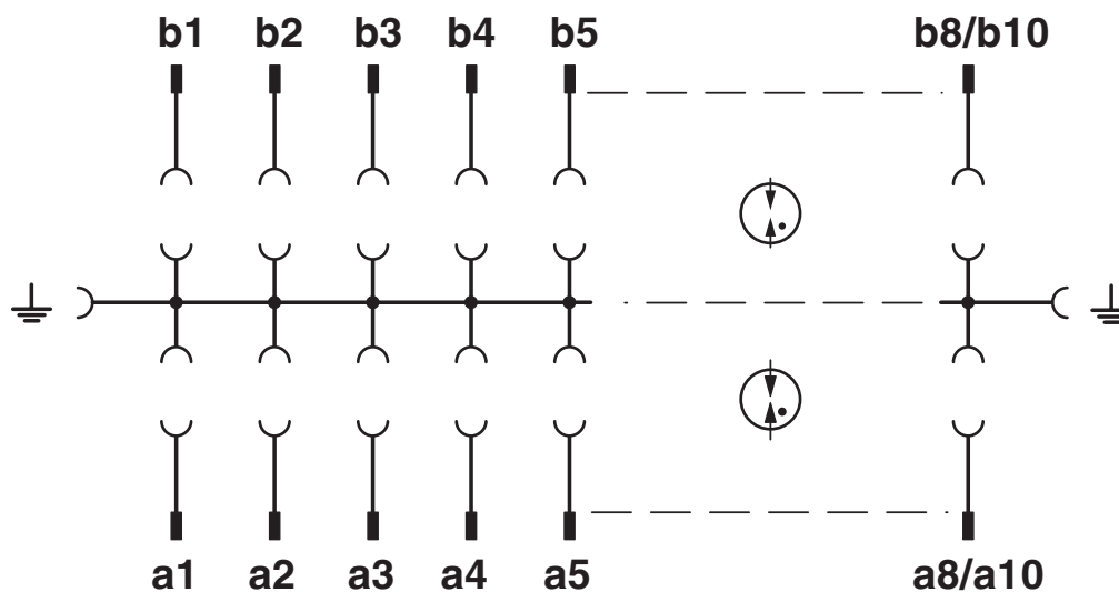
Circuit diagram
