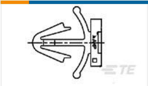
TE Part #936286-1 CLIP FOR 090III(7.0KEY HOLE)
