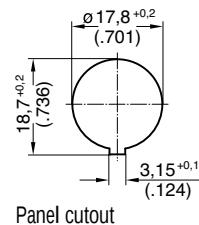
Panel cutout
