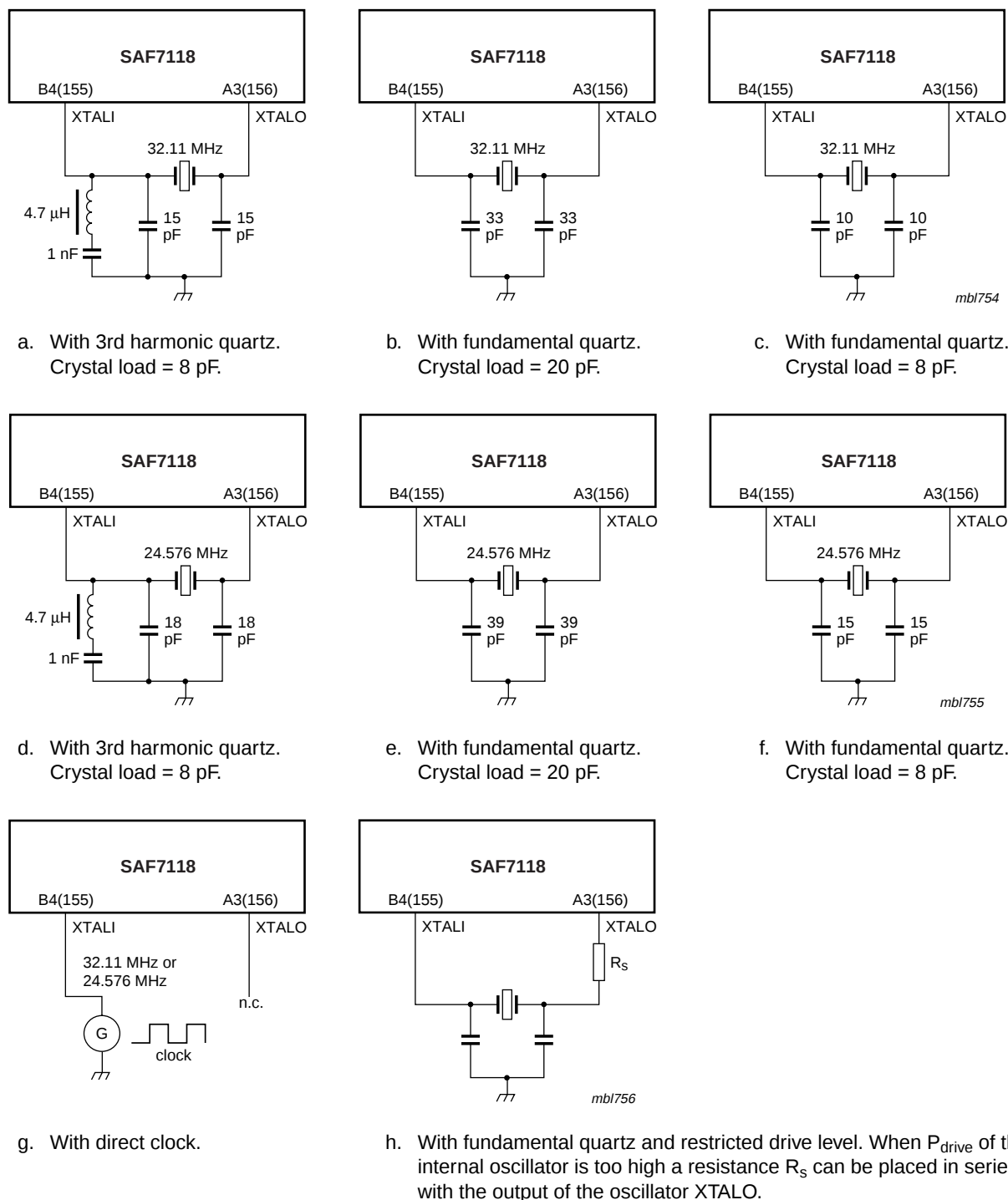
Fig 94. Oscillator application (pin numbers for QFP160 in parenthesis)
