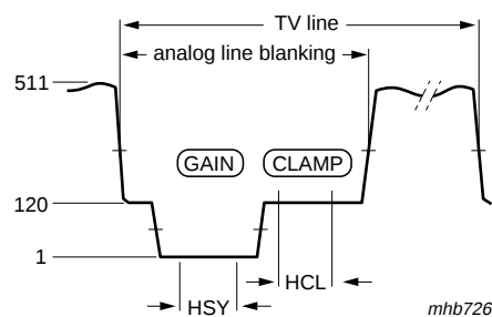
Fig 7. Analog line with clamp (HCL) and gain range (HSY)
