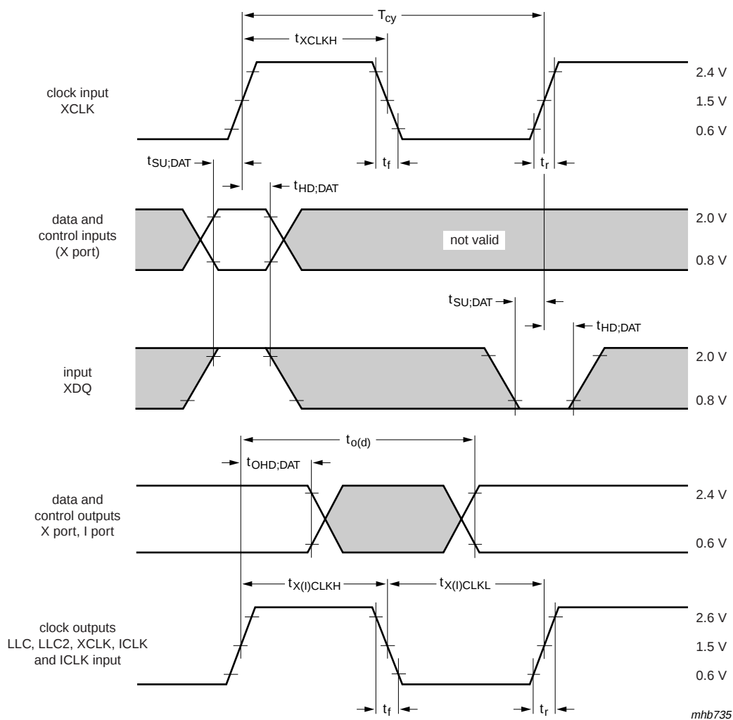
Fig 91. Data input/output timing diagram (X port, RT port and I port)
