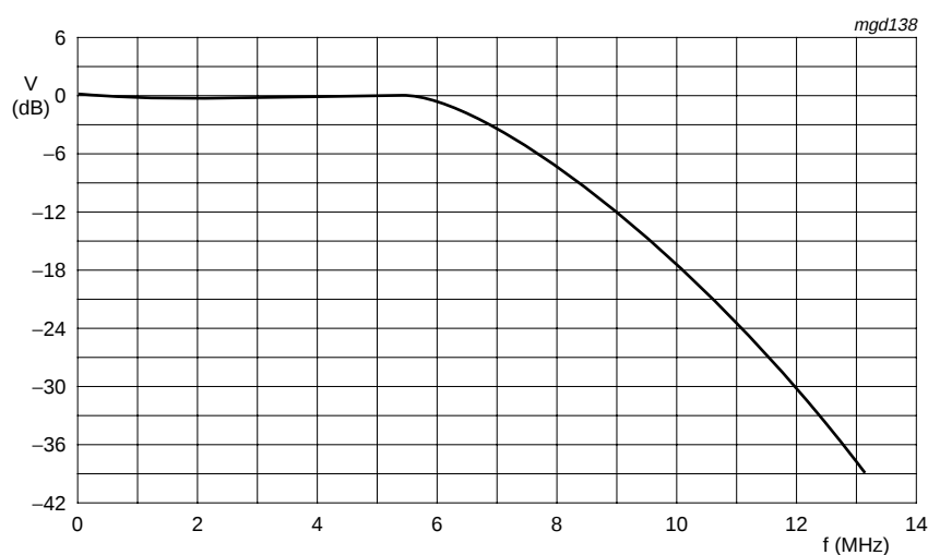
Fig 4. Anti-alias filter
