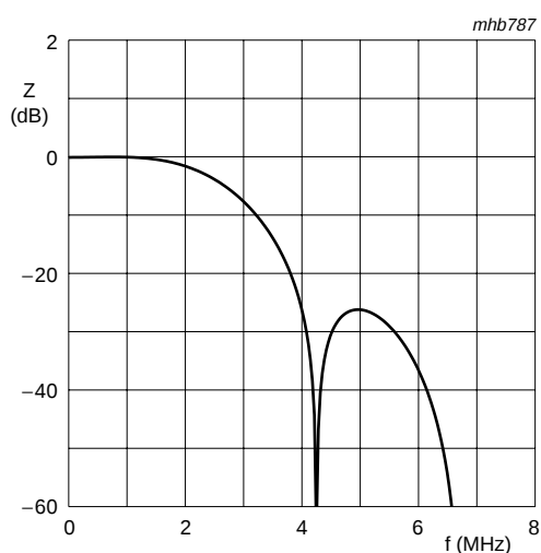
Fig 28. Y high-pass filter frequency response
