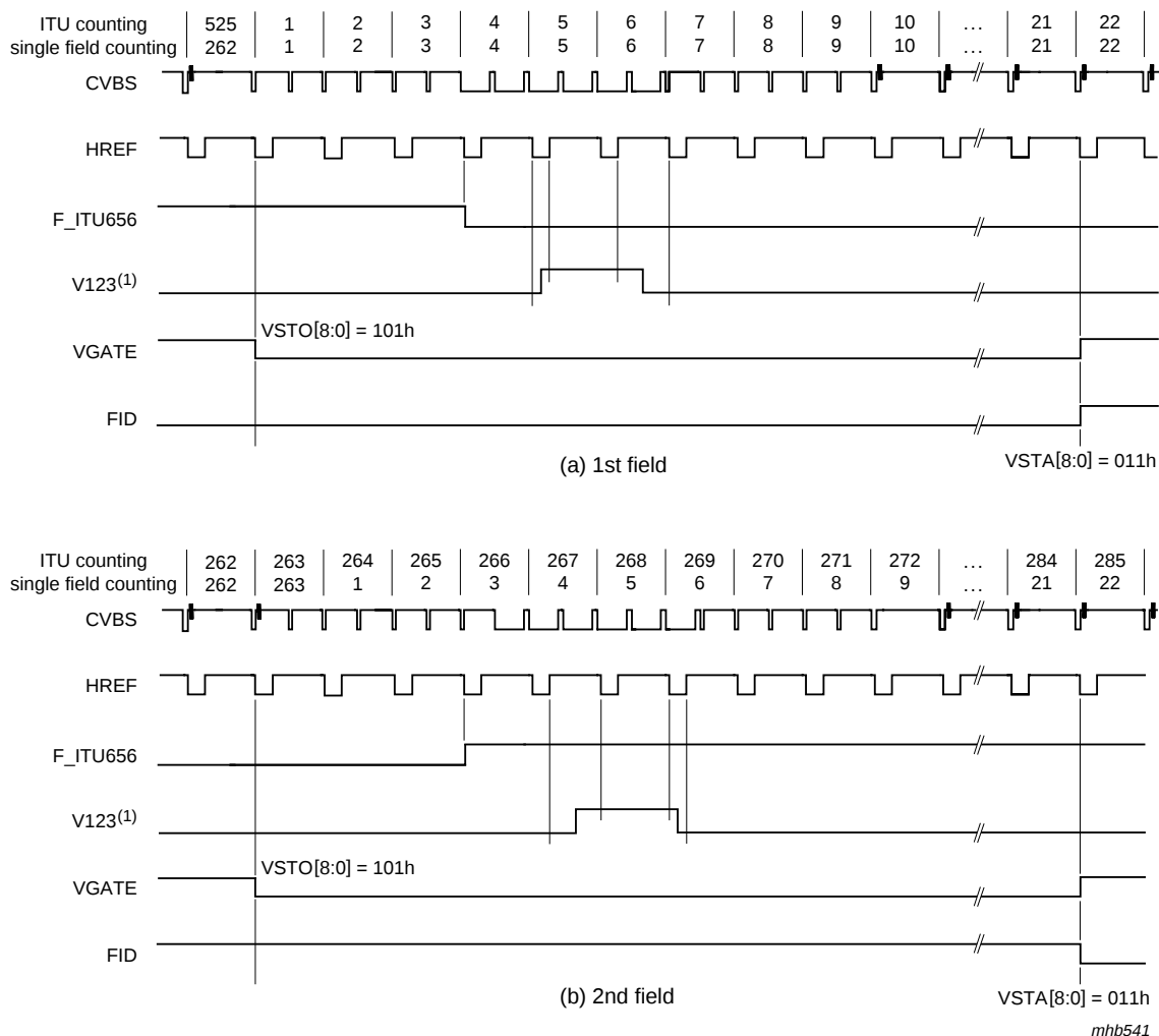
(1) The inactive going edge of the V123 signal indicates whether the field is odd or even. If HREF is active during the falling edge of V123, the field is ODD (field 1). If HREF is inactive during the falling edge of V123, the field is EVEN. The specific position of the slope is dependent on the internal processing delay and may change a few clock cycles from version to version. The control signals listed above are available on pins RTS0, RTS1, XRH and XRV according to Table 8 . For further information see Table 56 , Table 57 and Table 58 .
