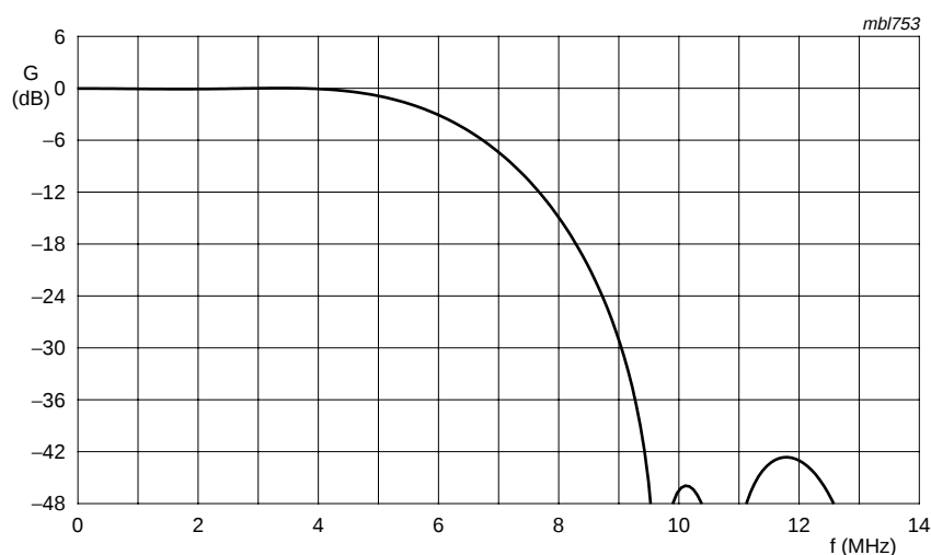
Fig 5. Decimation filter
