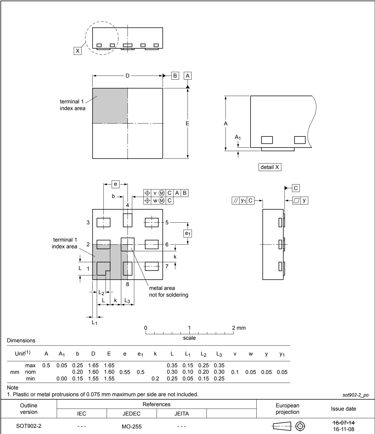
Figure 28. Package outline SOT902-2 (XQFN8)
