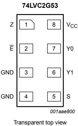
Figure 4. Pin configuration SOT833-1, SOT1089, SOT1116 and SOT1203
