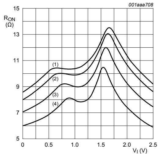
Figure 10. Typical ON resistance as a function of input voltage; T_{amb} = 25\text{ }^{\circ}\text{C}
