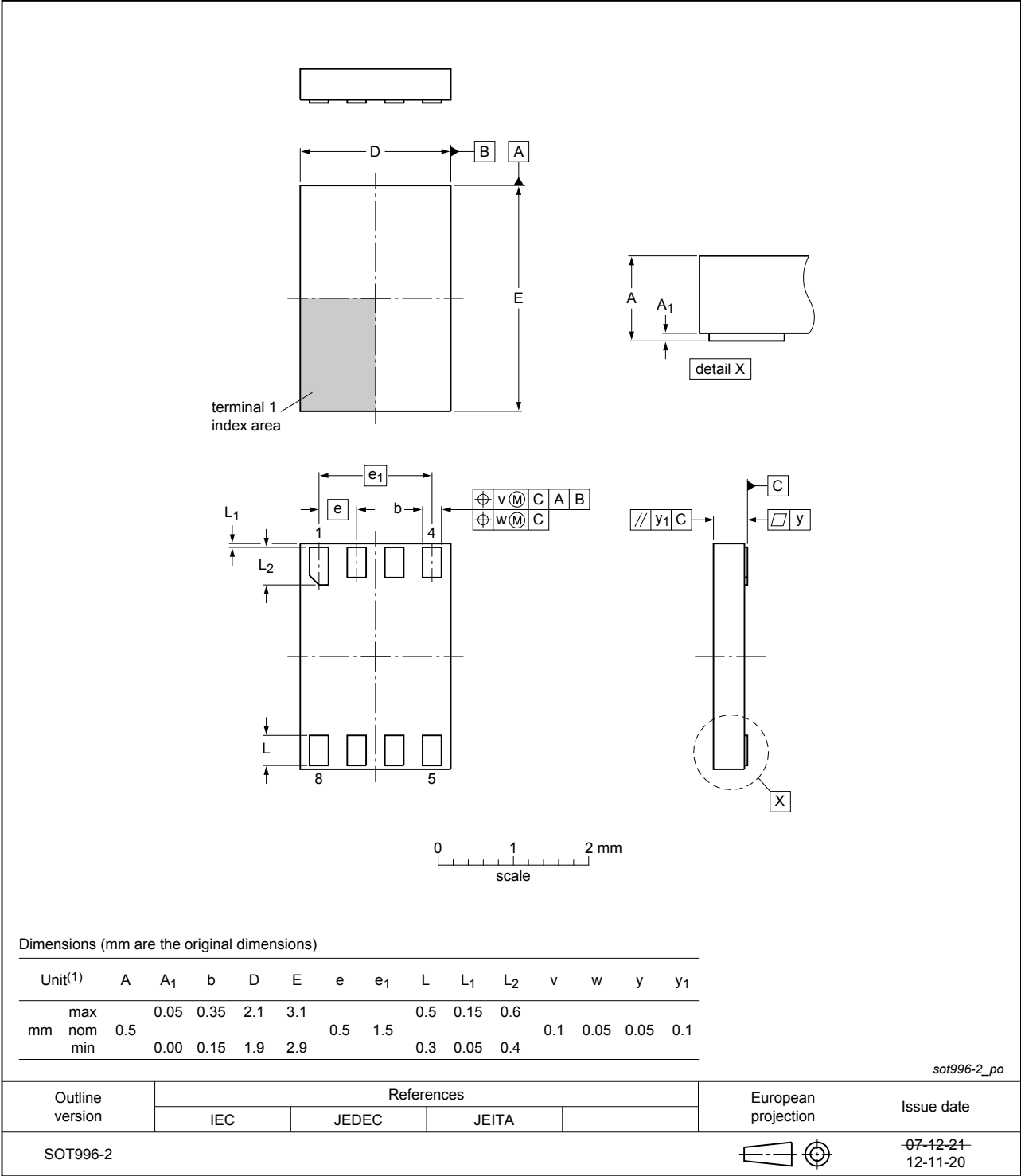
Figure 27. Package outline SOT996-2 (XSON8)
