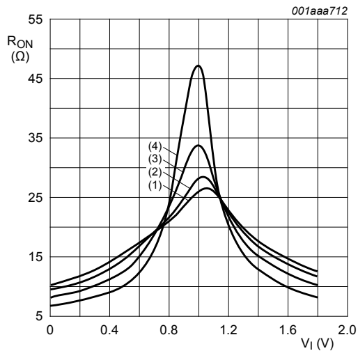
Figure 10. Typical ON resistance as a function of input voltage; T_{amb} = 25\text{ }^{\circ}\text{C}
