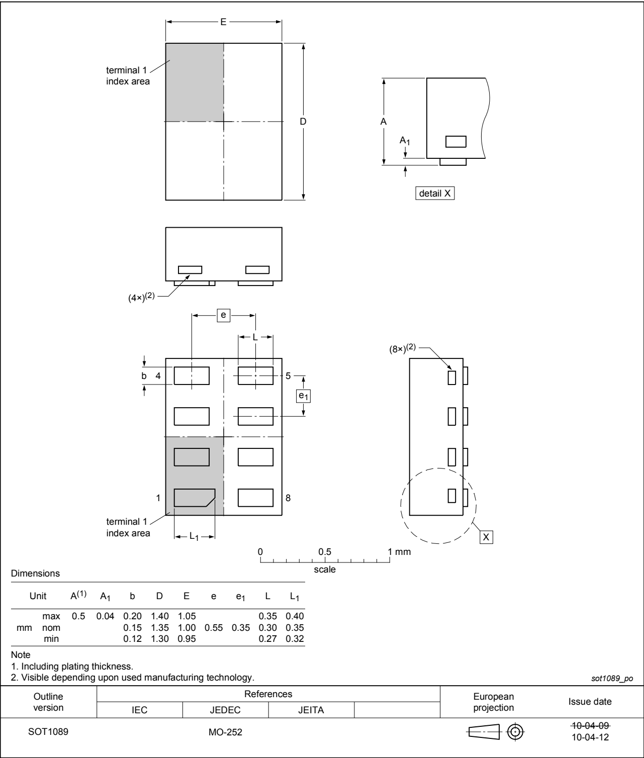
Figure 26. Package outline SOT1089 (XSON8)
