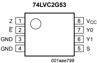
Figure 3. Pin configuration SOT505-2 and SOT765-1
