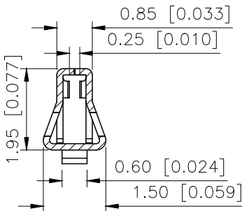
SECTION:C-C SCALE:1:1
