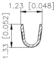
SECTION:B-B SCALE:1:1
