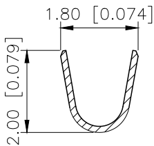
SECTION:A-A SCALE:1:1
