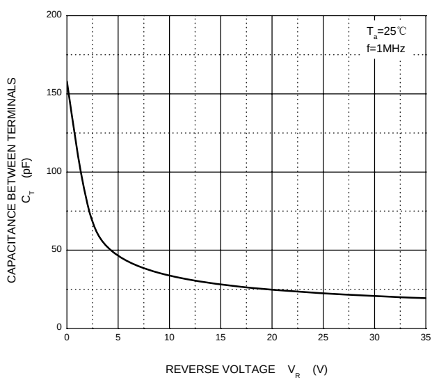
Capacitance Characteristics
