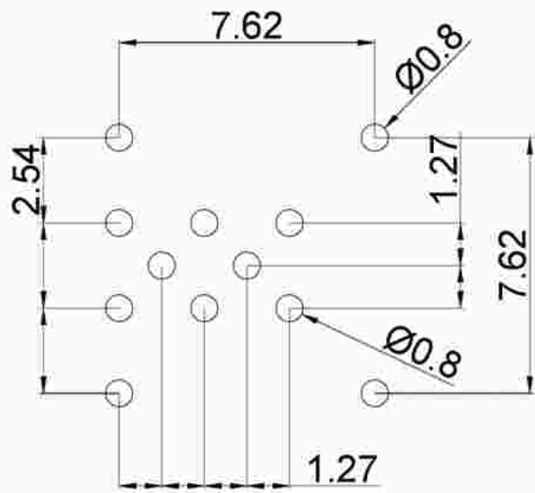
Pcb plate opening size (PCB板开孔尺寸)
