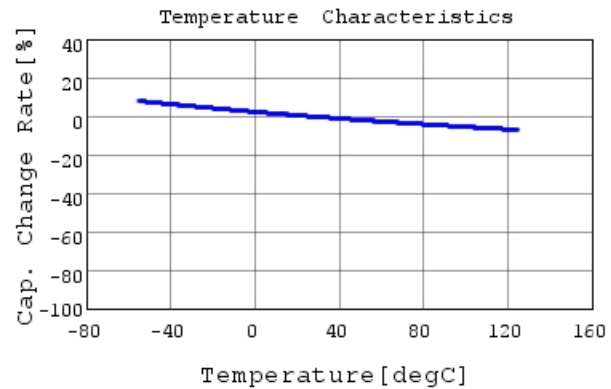
RCE7U2E102J1M1H03A C-Temp. capchange, DCOV,
