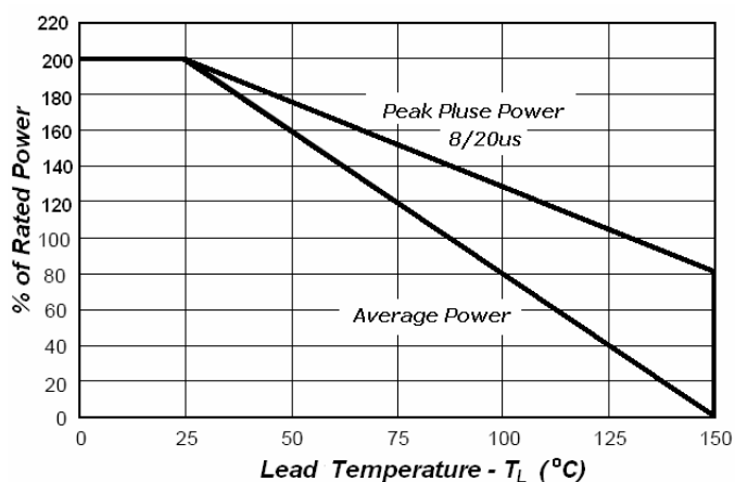
Fig2.Power Derating Curve
