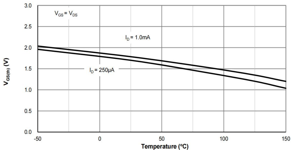
Figure 5: V_{GS(th)} vs. Junction Temperature
