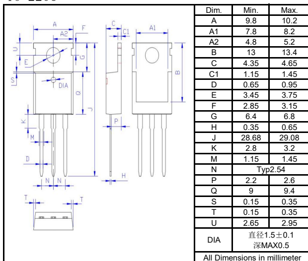
TO-220C
