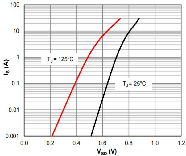
Figure 7: Body-Diode Characteristics
