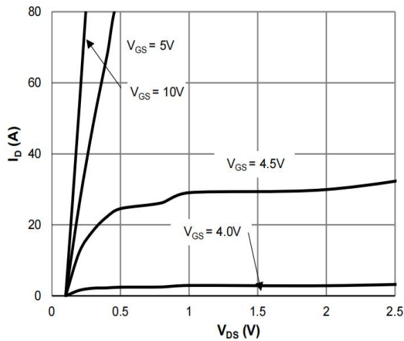
Figure 1: Saturation Characteristics
