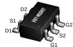
SOT-23-6L (TSOP-6-1.5mm)
