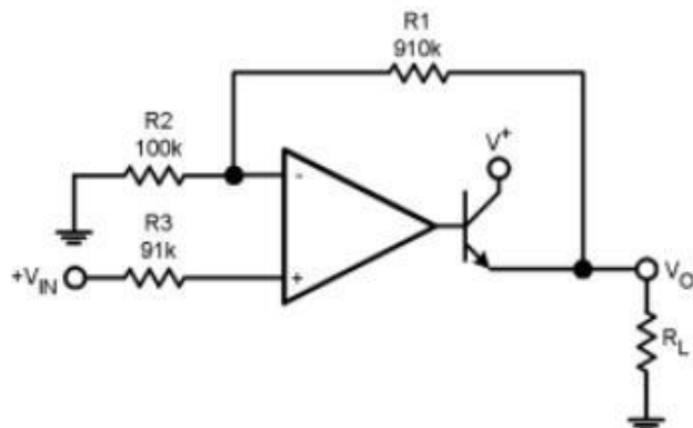
Power Amplifier
