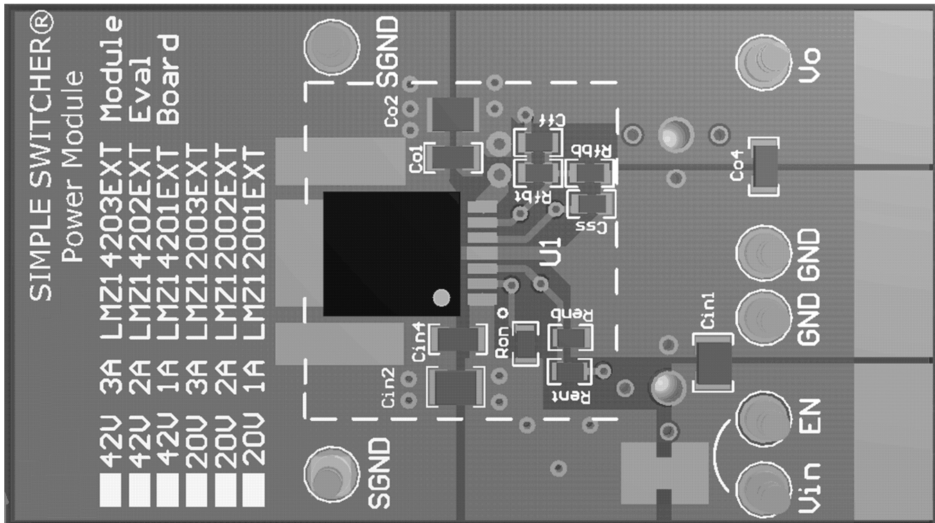
Figure 37. Top View of Board
