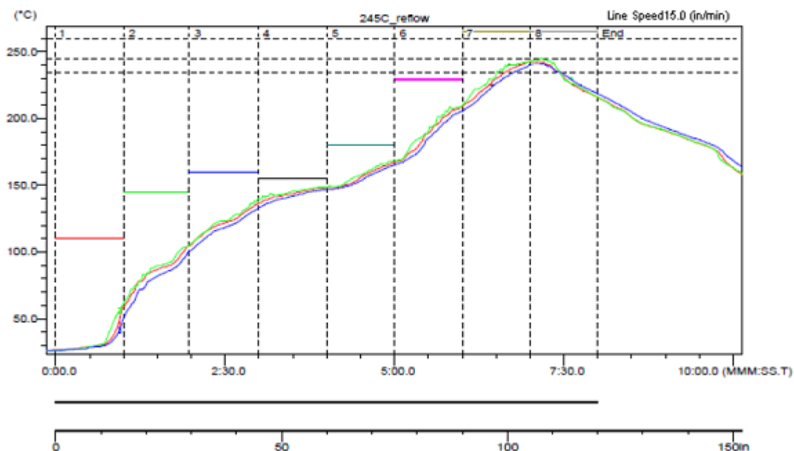
Figure 39. Sample Reflow Profile
