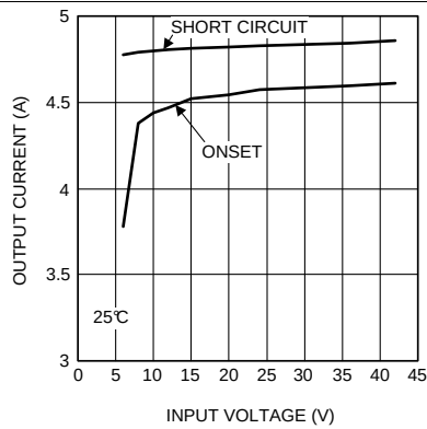
Figure 25. Current Limit 3.3 V_{OUT} at 25^\circ\text{C}
