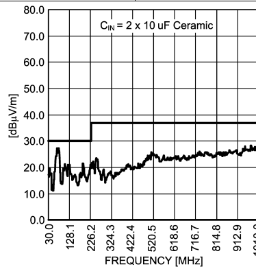
Figure 34. Radiated Emissions (EN 55022 Class B) from Evaluation Board
