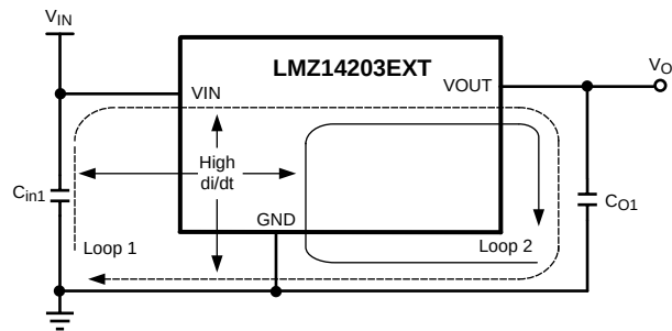
Figure 35. Critical Current Loops to Minimize
