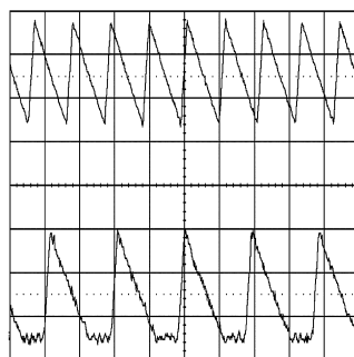
Figure 30. CCM and DCM Operating Modes V_{IN} = 24 \text{ V} , V_O = 3.3 \text{ V} , I_O = 2 \text{ A} / 0.32 \text{ A} 2 \mu s/div
