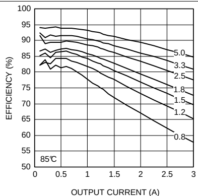
Figure 9. Efficiency 6-V Input at 85°C
