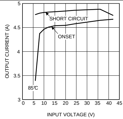
Figure 26. Current Limit 3.3 V_{OUT} at 85^\circ\text{C}
