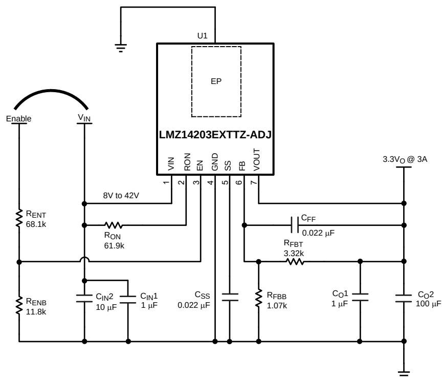
Figure 29. Evaluation Board Schematic Diagram
