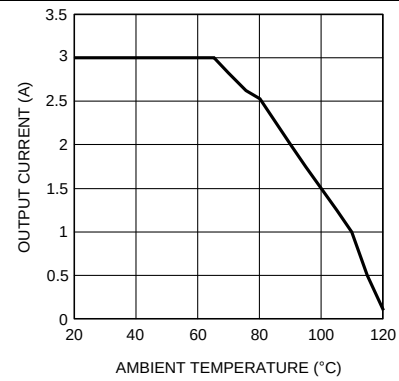
Figure 33. Thermal Derating Curve V_{IN} = 24\text{ V} , V_{OUT} = 5.0\text{ V}
