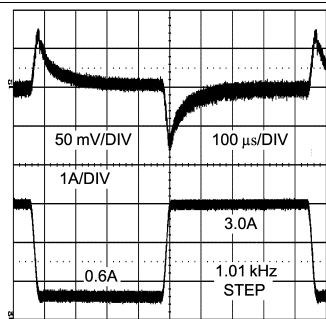
Figure 21. Line and Load Regulation at -55°C
