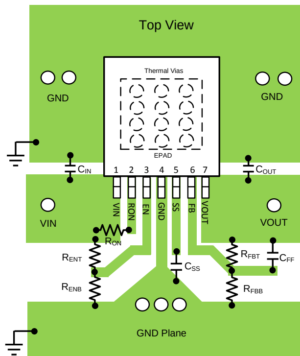
Figure 36. PCB Layout Guide
