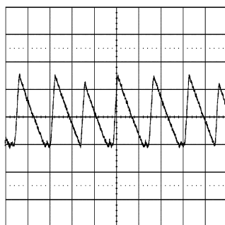
Figure 31. Transition Mode Operation V_{IN} = 24 \text{ V} , V_O = 3.3 \text{ V} , I_O = 0.35 \text{ A} 2 \mu s/div
