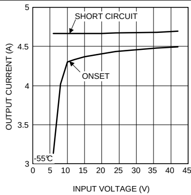
Figure 27. Current Limit 3.3 V_{OUT} at -55^\circ\text{C}
