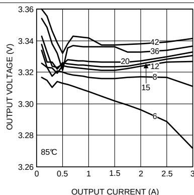
Figure 20. Line and Load Regulation at 85°C
