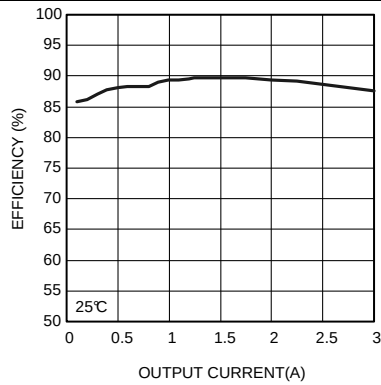
Figure 32. Efficiency V_{IN} = 24\text{ V} V_{OUT} = 5.0\text{ V}
