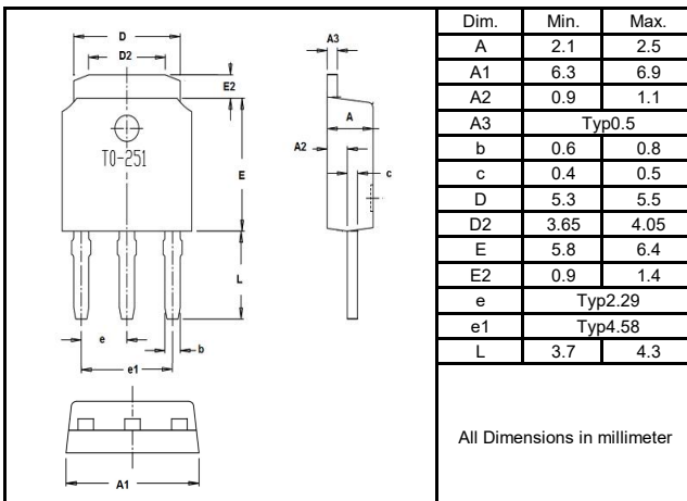
T0-251
