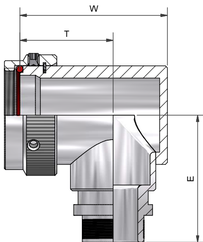
90° BACKSHELL - TYPE 1
