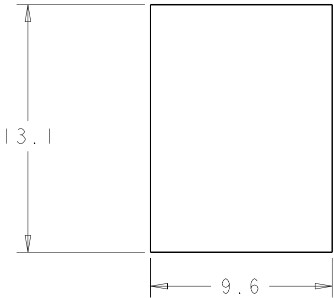
SUGGESTED PANEL CUTOUT MAX PANEL THICKNESS 1.7
