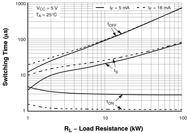
Figure 9. Switching Time vs. Load Resistance (FODM121/2701/2705)
