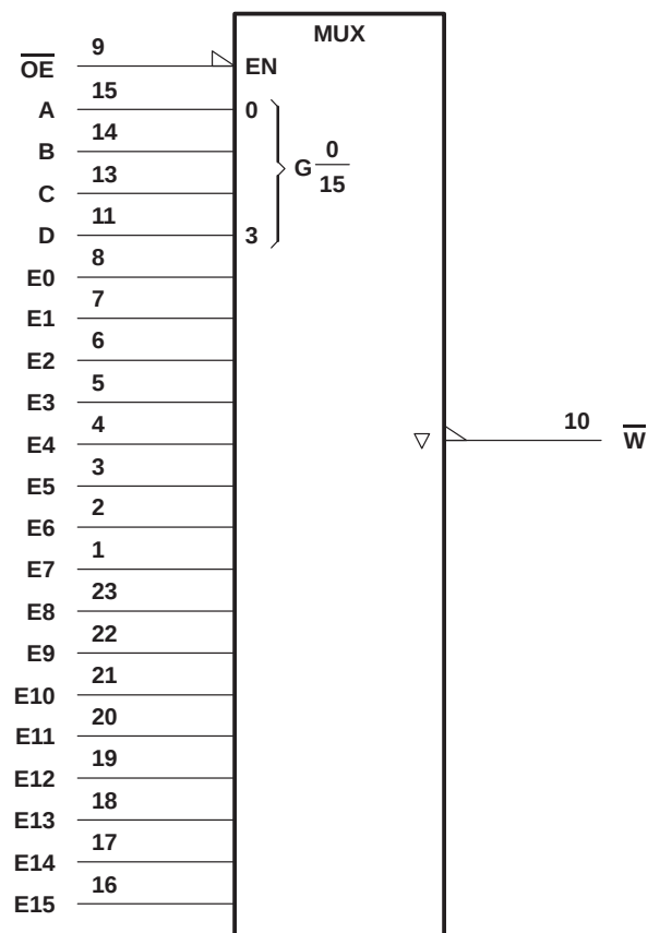
logic symbol†
