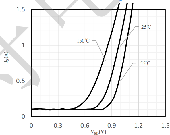
Fig 4 Body-Diode Characteristics
