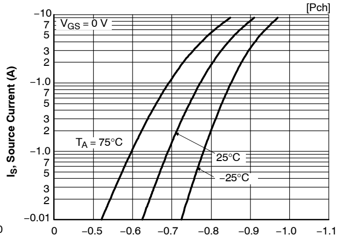
Figure 17. I_S - V_{SD}
