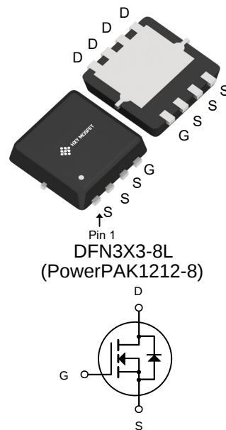
N-Channel MOSFET
