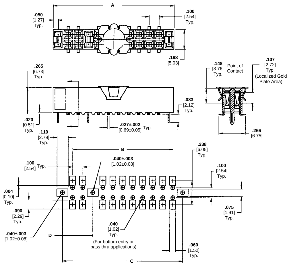
Recommended PC Board Layout (.008 [0.20] thick stencil)
