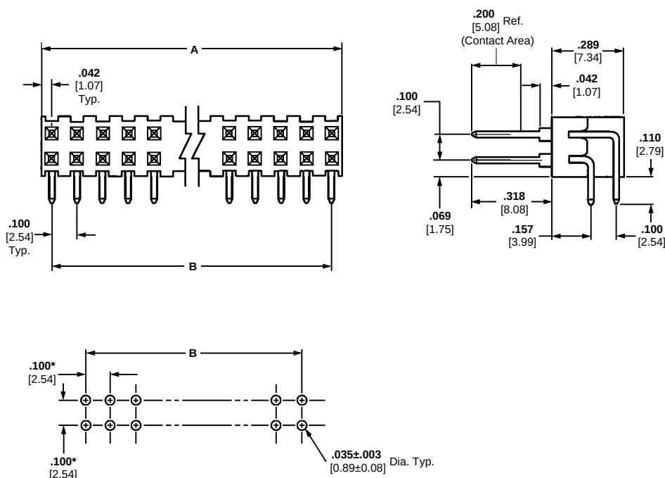
Recommended PC Board Hole Layout (for .055 [1.40] min. thick PC board)
