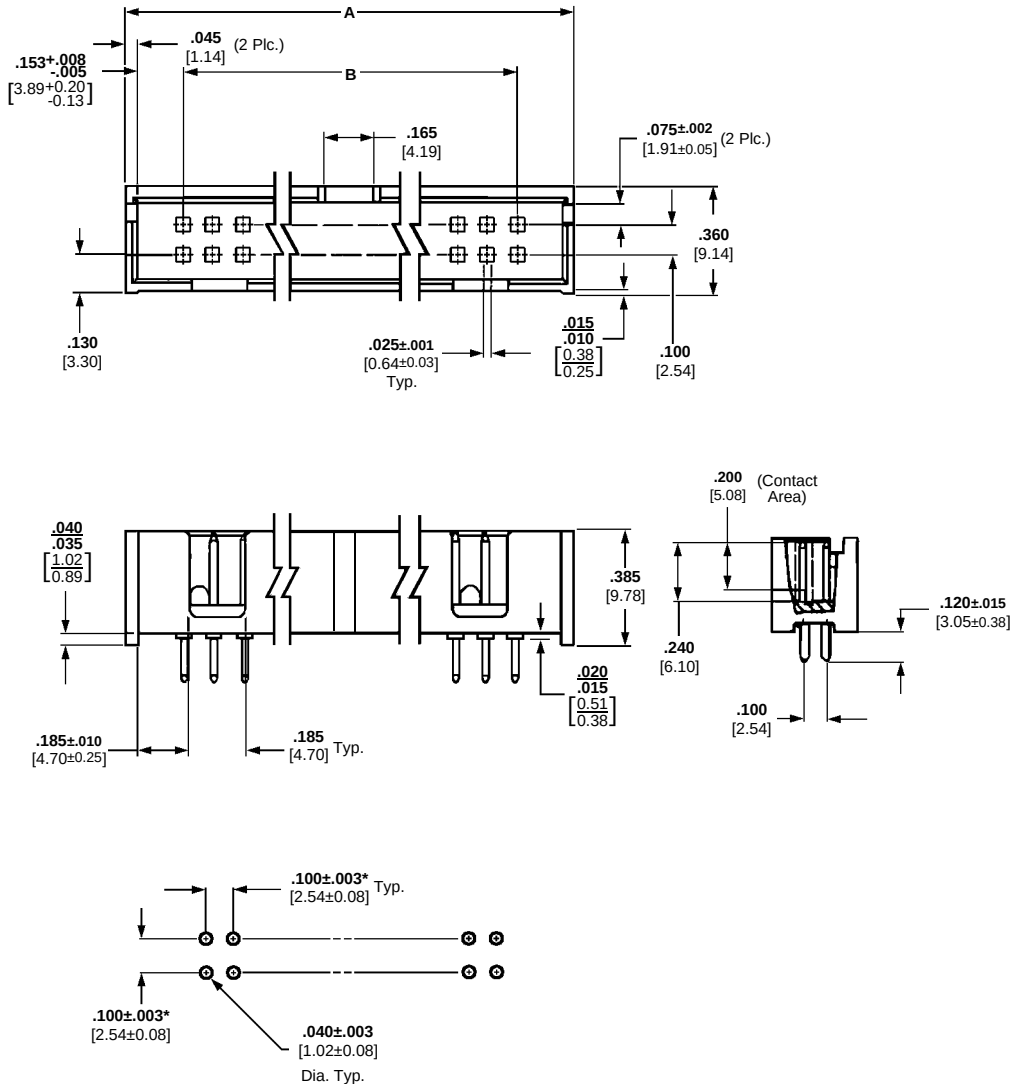
Recommended PCBoard Hole Layout For Manual Insertion
