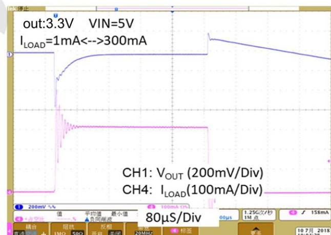
Load Transient Response II
