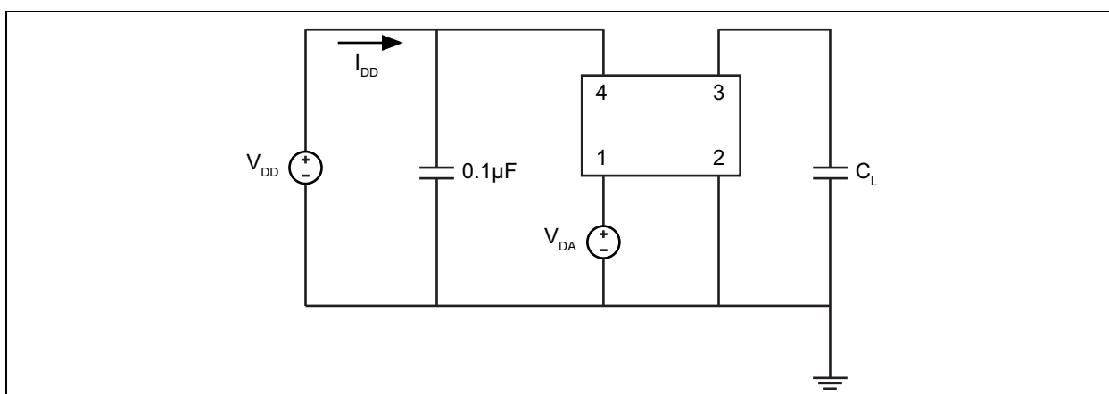
FIGURE 3-2: Test Circuit.
