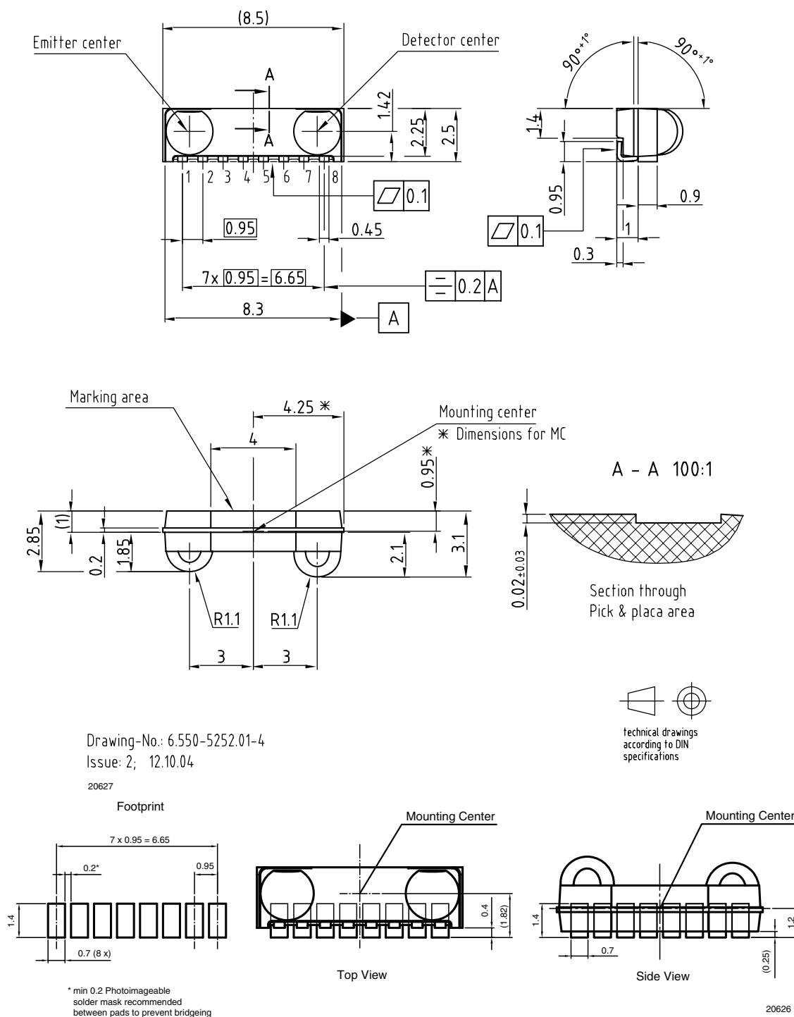
Fig. 8 - Package Drawing
