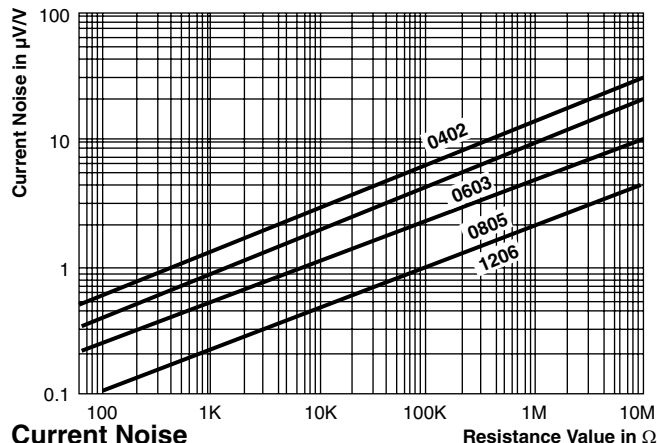
Current Noise
