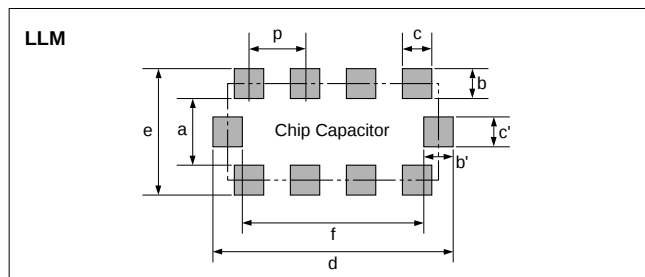
Part Number Dimensions (mm) a b, b' c, c' d e f p LLM21 0.6 to 0.8 (0.3 to 0.5) 0.3 2.0 to 2.6 1.3 to 1.8 1.4 to 1.6 0.5 LLM31 1.0 (0.3 to 0.5) 0.4 3.2 to 3.6 1.6 to 2.0 2.6 0.8
