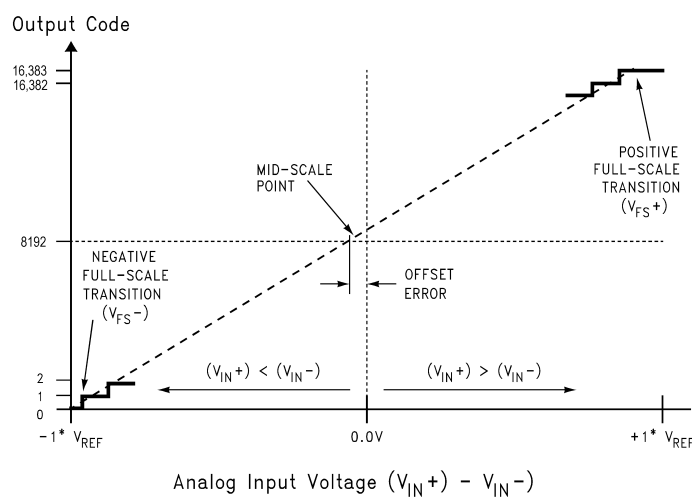
Figure 3. Transfer Characteristic
