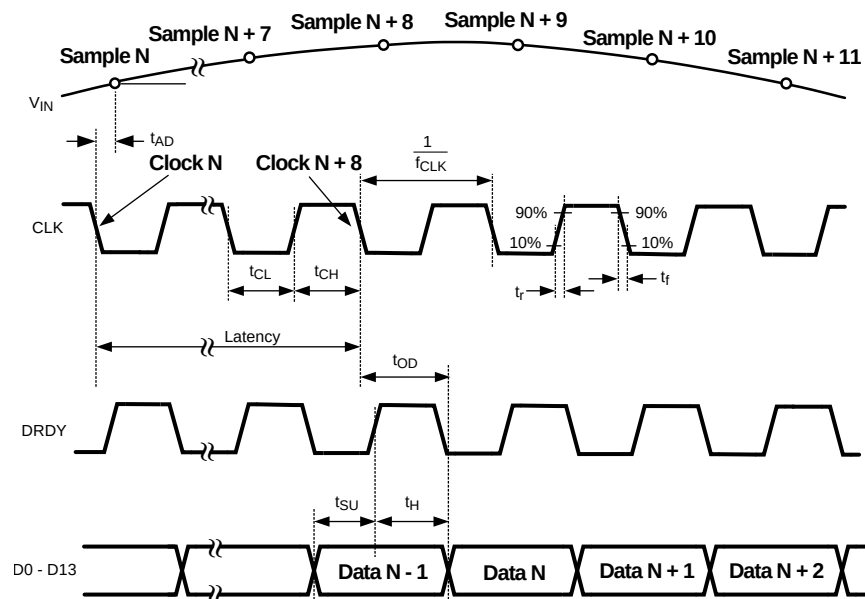
Figure 2. Output Timing
