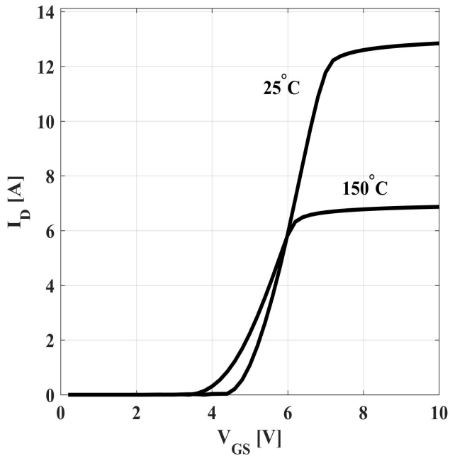
Figure 11: Typ. Transfer Characteristics
