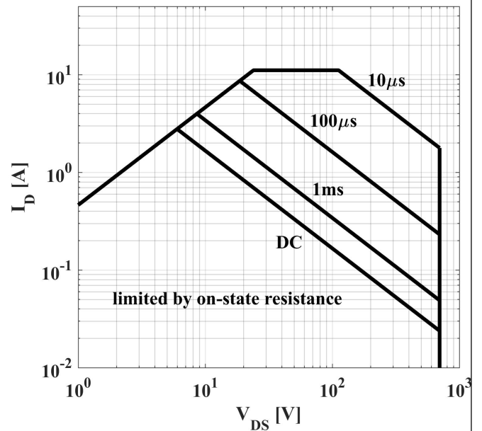
Figure 6: Safe Operating Area
